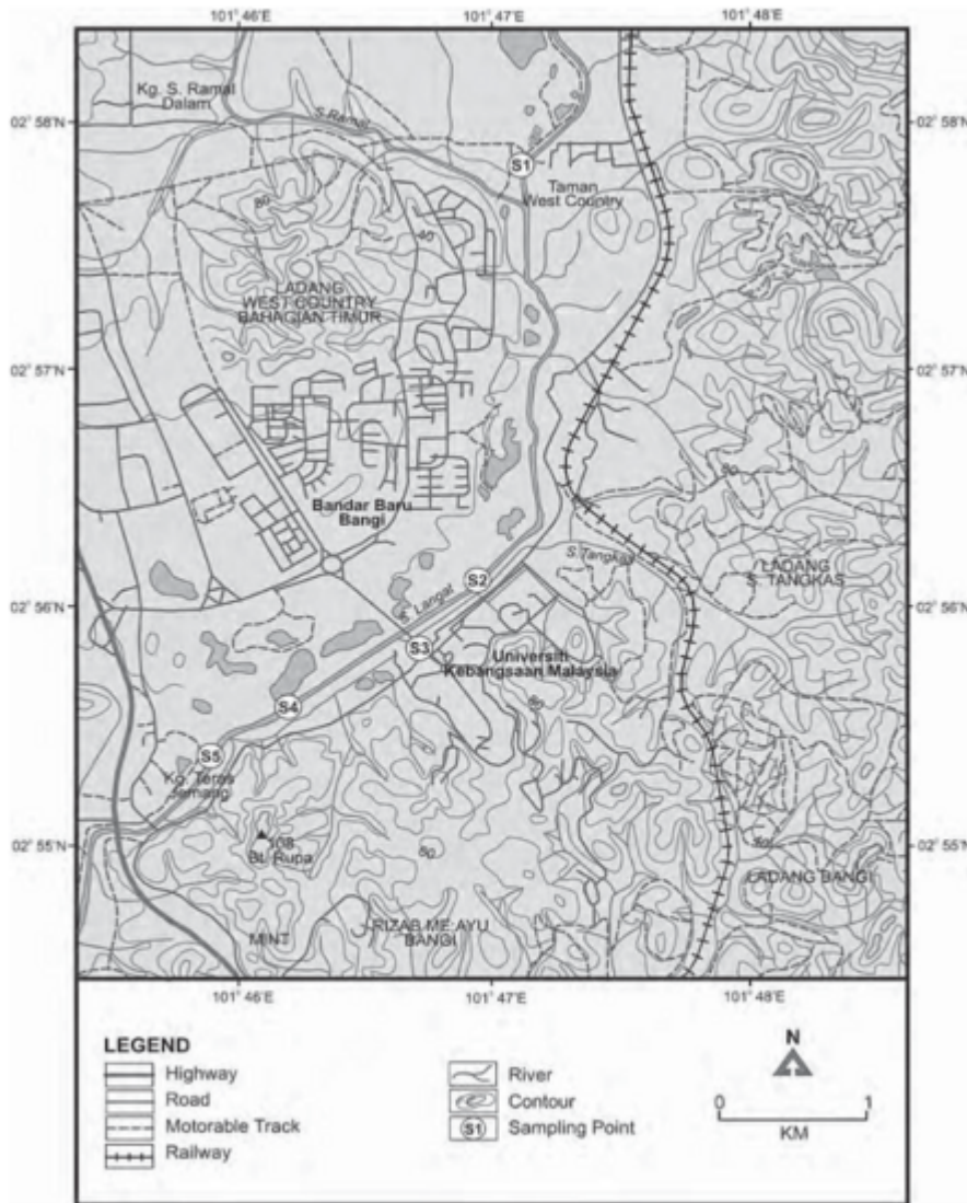
FIGURE 1 Locations of five sampling stations along the Langkat River
